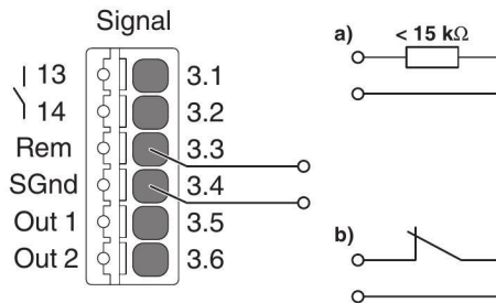
Figure 20 SLEEP MODE connection versions
