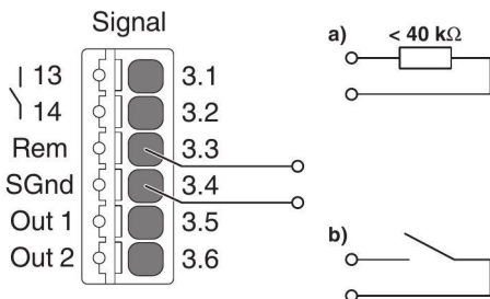
Figure 34 External wiring versions, disable SLEEP MODE
