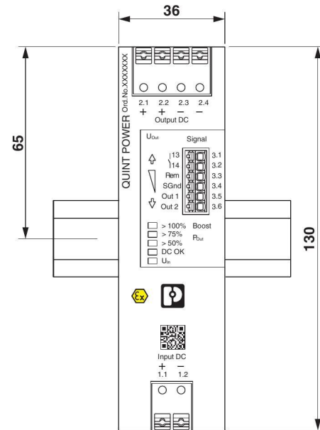
Figure 3 Device dimensions (dimensions in mm)
